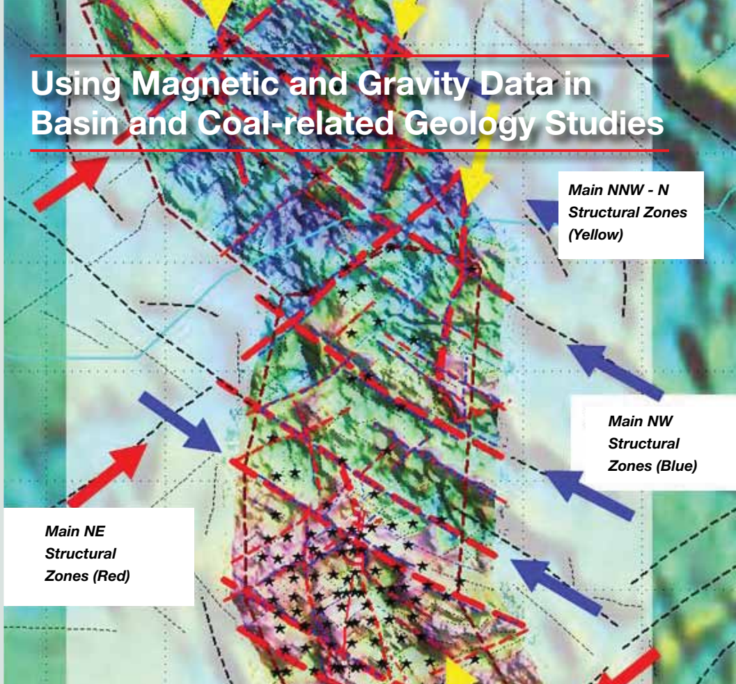
Regional magnetics overlain by the detailed magnetic survey data
