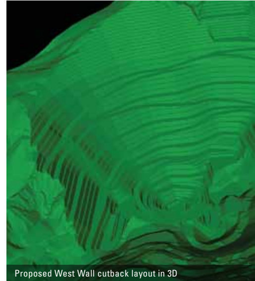
Proposed West Wall cutback layout in 3D
