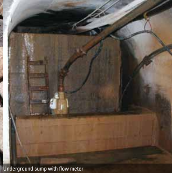
Underground sump with flow meter
