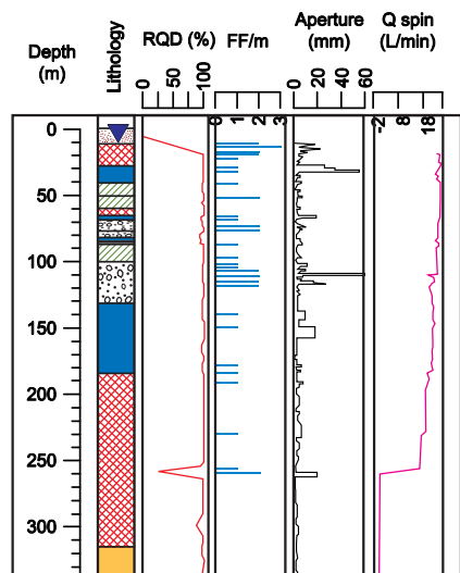
Core log with spinner test results
