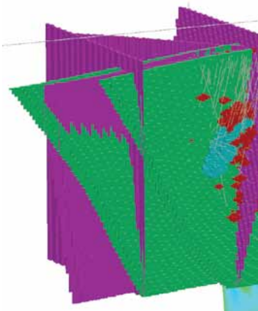
Juno1 (left): Geological block model showing fold axis, faults, assays and ore shoot. Juno2 (right): Sections and plan showing different prospectivity within the geological block model.
