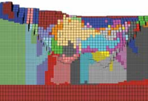
FLAC3D model cross-section showing cohesion in kPa, looking west
