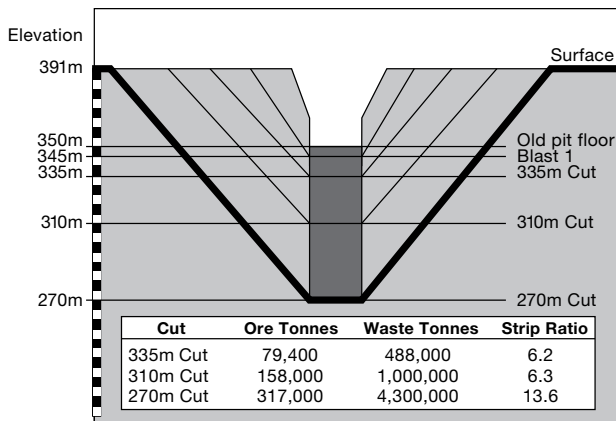
Figure 1: Comparison of the open pit and vertical pit scenarios
