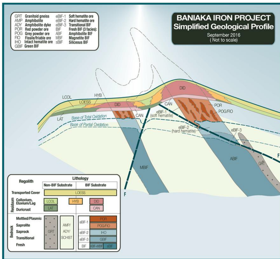
Figure 1: Schematic geological model of detrital iron in the Baniaka Project, Gabon
