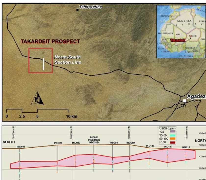
Figure 3: Location and cross-section through the Takardeit uranium mineralisation, showing gently-dipping tabular nature of the deposit (section from NGM, 2010)
