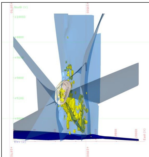
Figure 4: Preliminary modelled gold grade shell (yellow) and fault architecture (blue) illustrating southeast plunge of gold mineralisation along intersecting fault structure.
